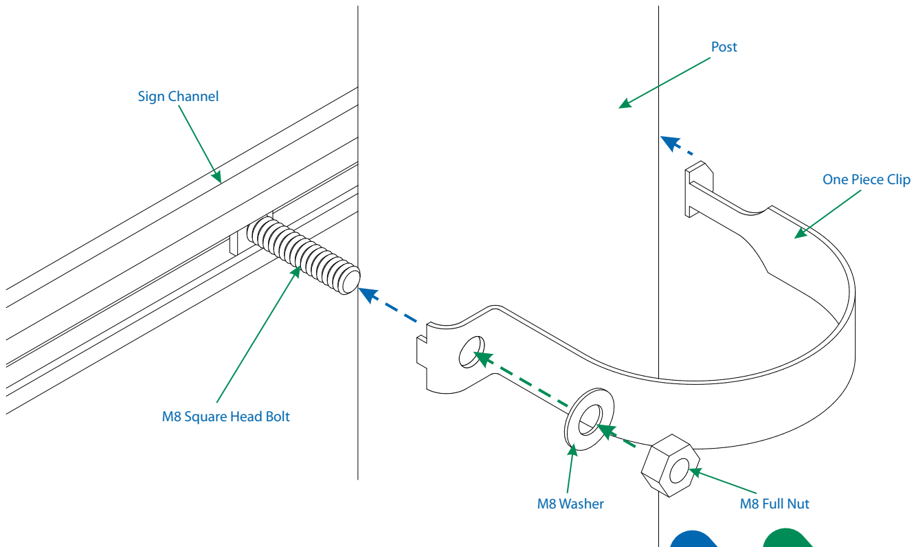
OPC - One Piece Clips in various colour options
