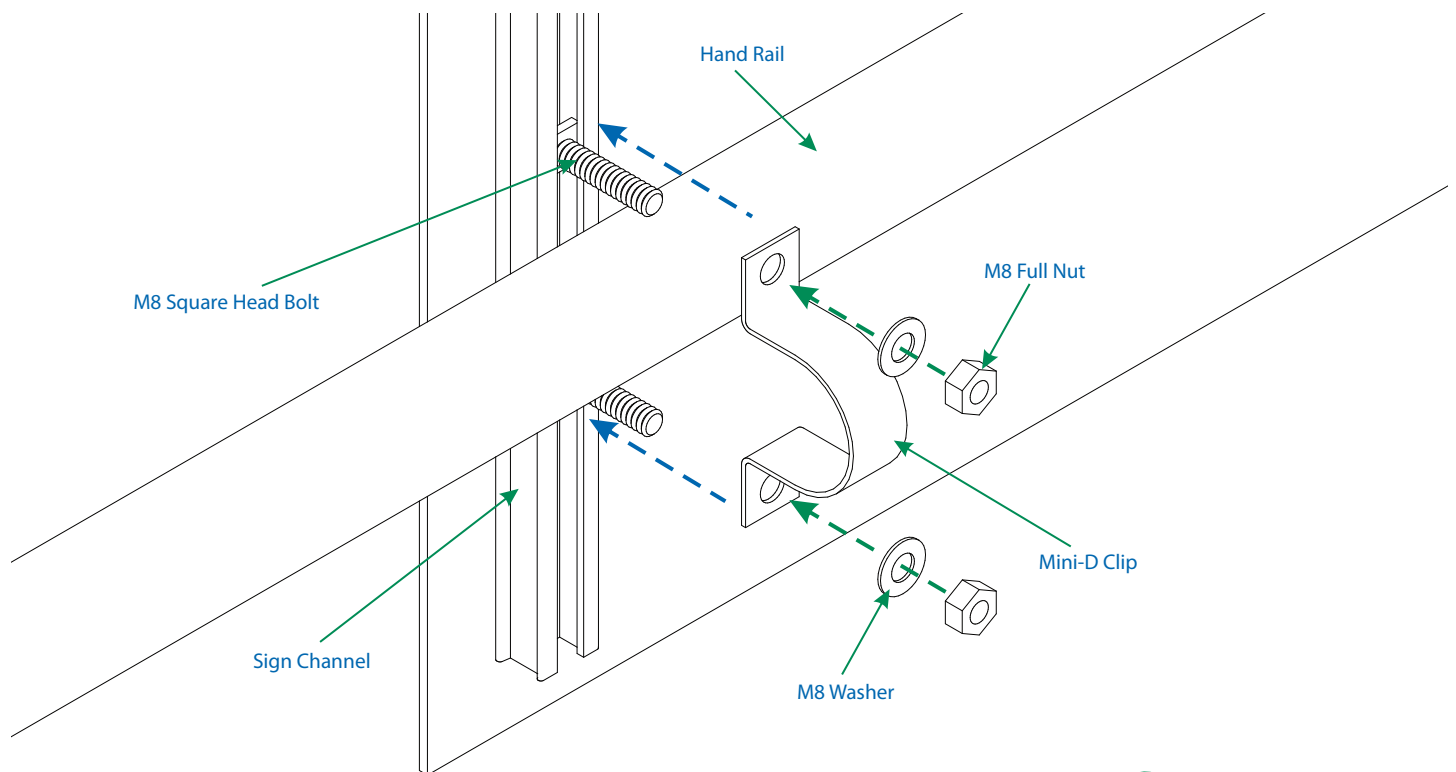
MDC - Mini-D Clips in self colour and painted options
