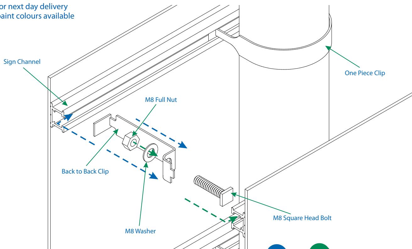
BBC - Back to Back Clips in self colour and painted options
