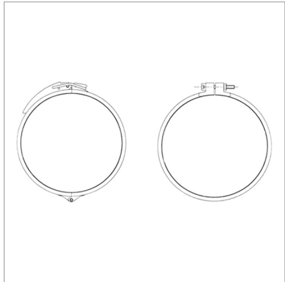
Rapid lock pull ring - with hinge and handle up to Ø400 mm. With bolt Ø450 mm and bigger.
