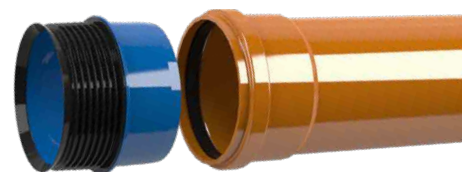
Direct connection with KG socket
